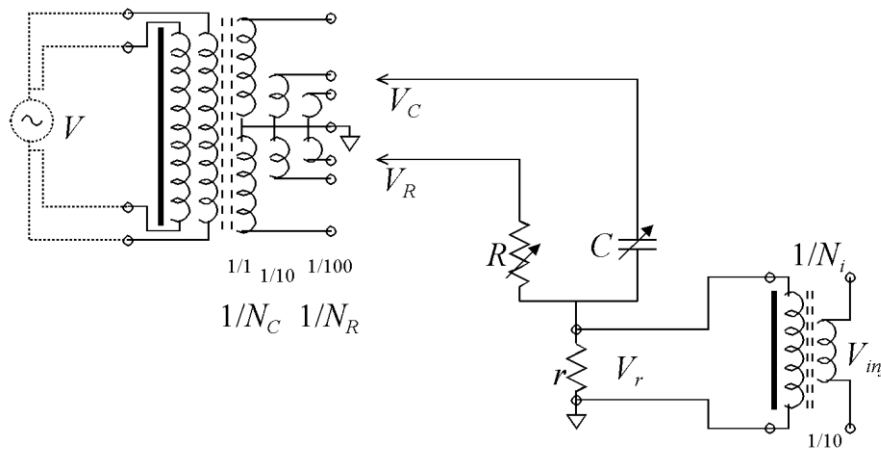
Figure A2.1. Schematic diagram of the voltage injection system
