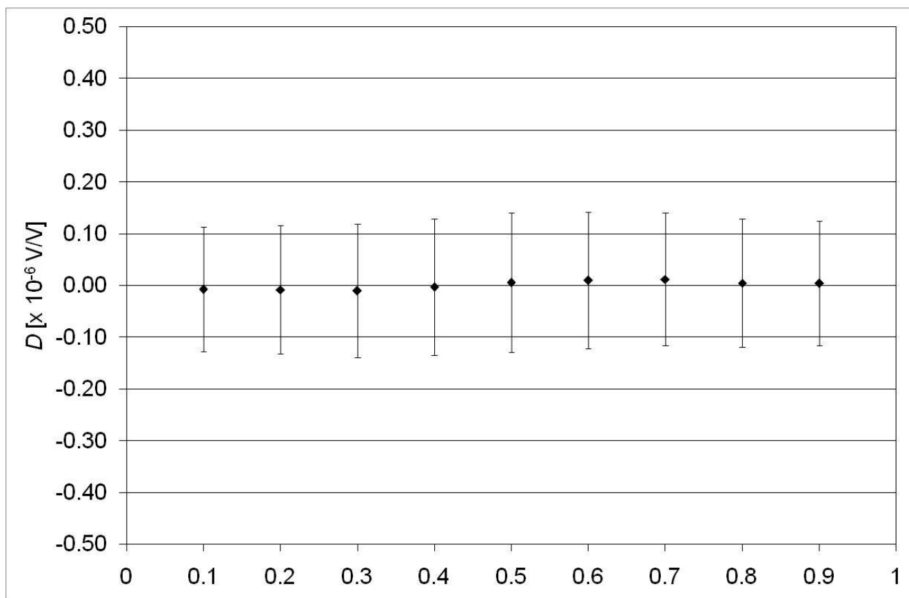
Figure 4. Degrees of equivalence at 400 Hz in phase
