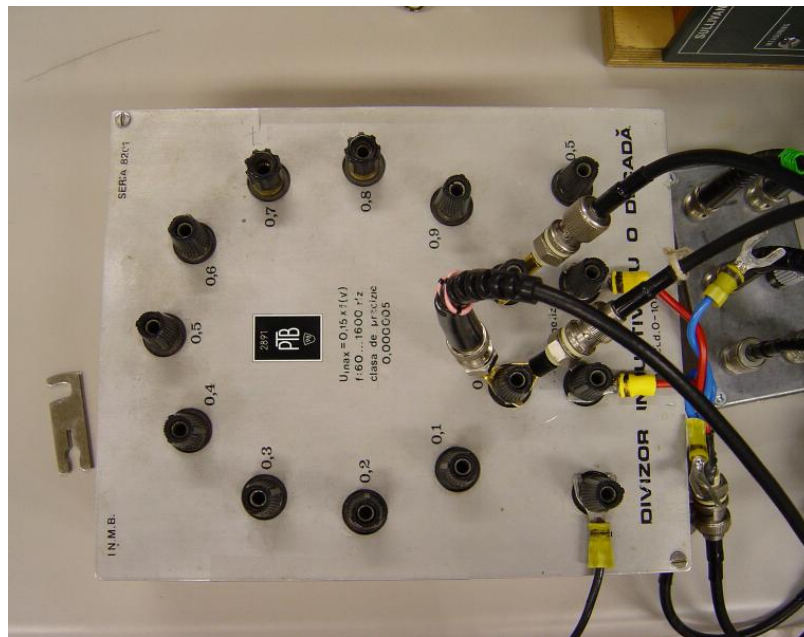
Figure 1. Travelling standard
