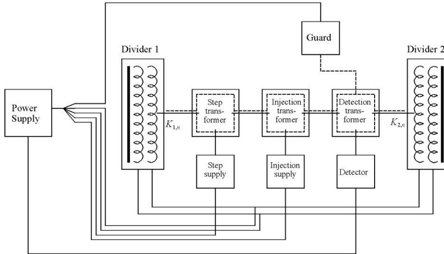
Figure A1.1. Schematic diagram of the measurement set-up
