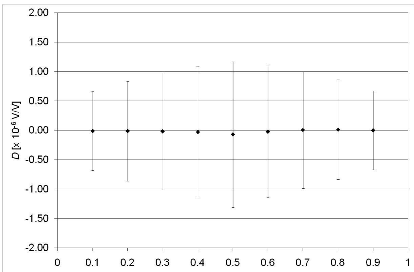
Figure 3. Degrees of equivalence at 55 Hz in quadrature
