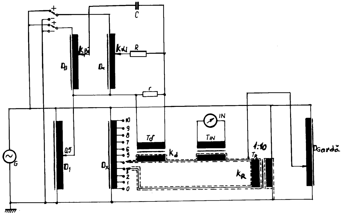
Figure A1.2. Schematics of the INM installation of voltage ratio measurement method by means of reference voltage method
