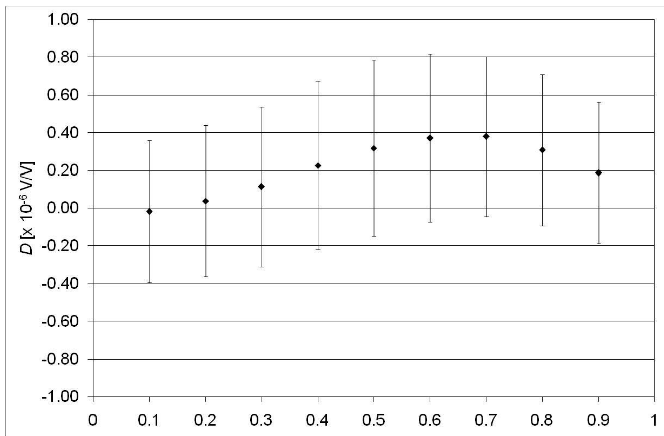
Figure 7. Degrees of equivalence at 1 kHz in quadrature
