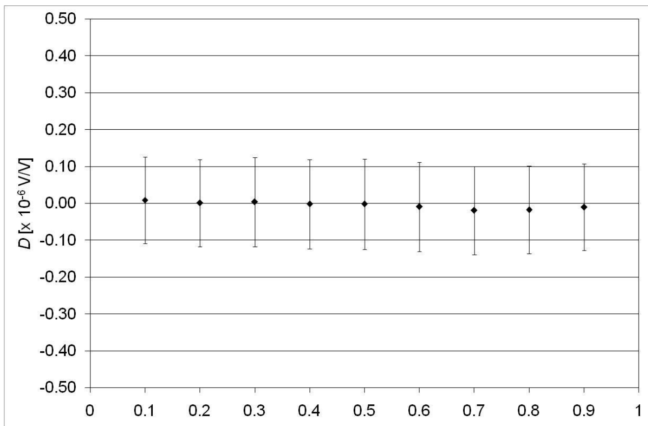
Figure 6. Degrees of equivalence at 1 kHz in phase
