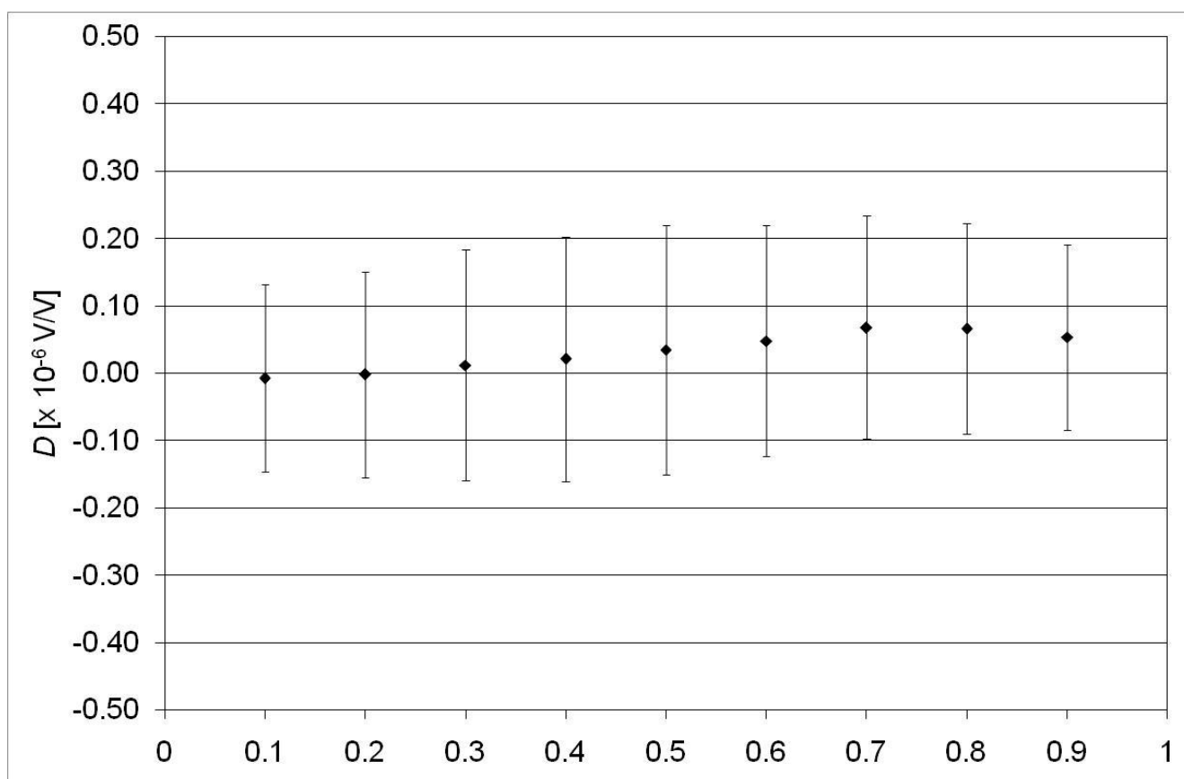
Figure 2. Degrees of equivalence at 55 Hz in phase
