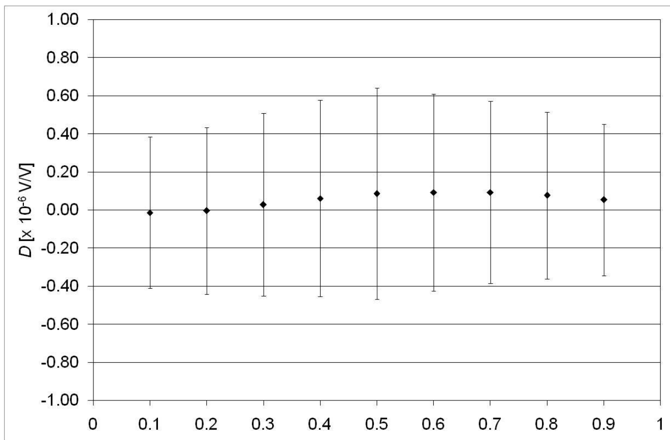
Figure 5. Degrees of equivalence at 400 Hz in quadrature
