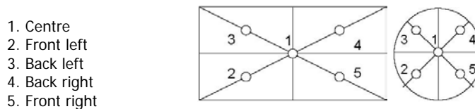
Fig. 5.3-1 Positions of load for test of eccentricity
