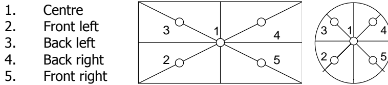
Figure 5.3-1 Positions of load for test of eccentricity
