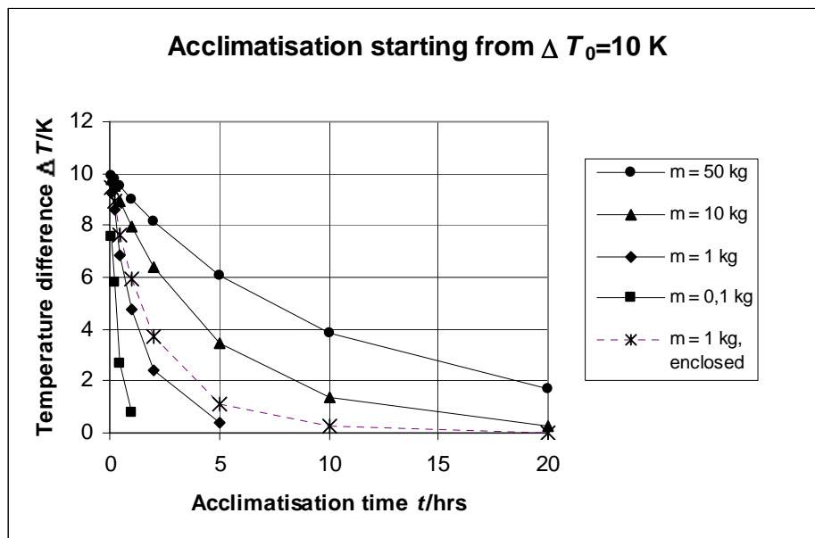
Figure F1.1: Acclimatisation of standard weights
