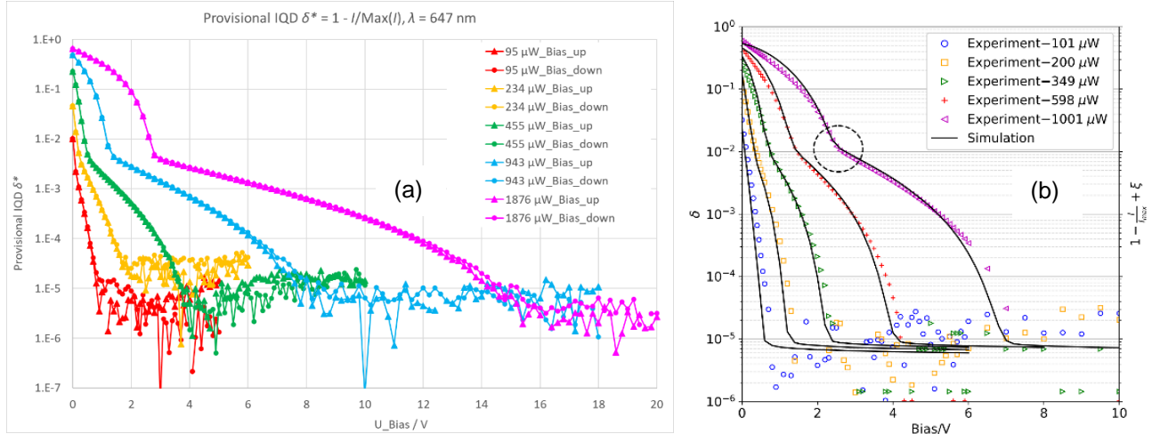
Figure 2-5. Comparison between I-V measured curves at 647 nm of chipS·CALE photodiodes (a) and qu-candela photodiodes (b).
