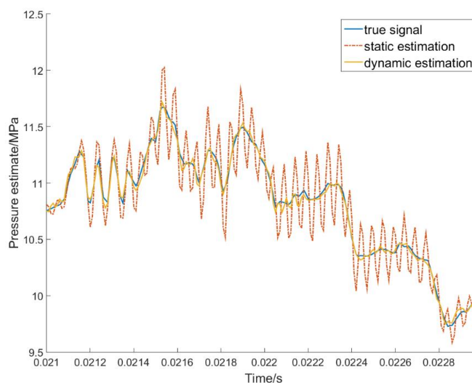
Figure 1: Estimating the value of a dynamic signal. The figure shows the effect of ignoring the dynamic properties of a measuring system compared to taking dynamic effects into account.
