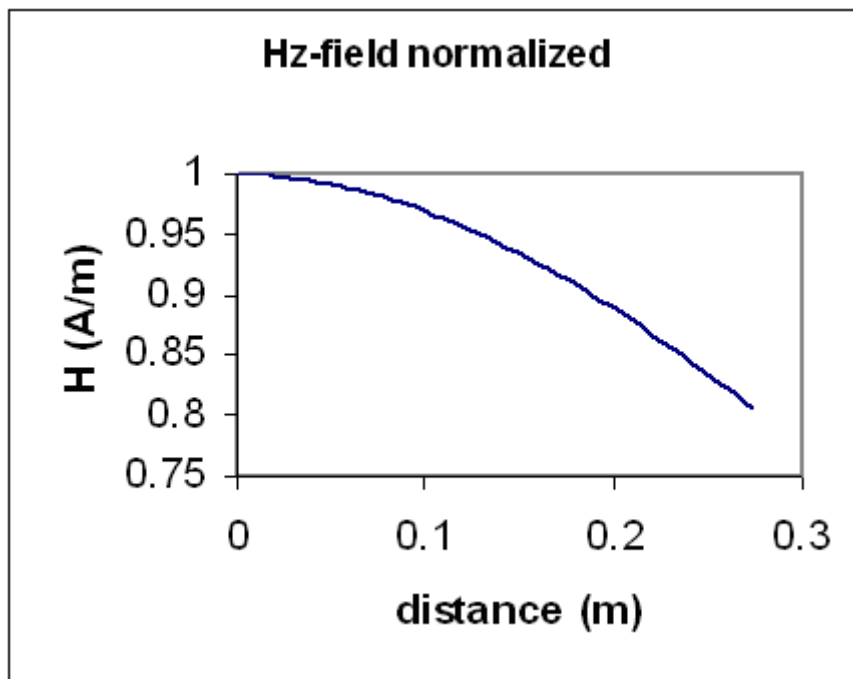
Fig 2 : Representation of Hz field according to the distance
